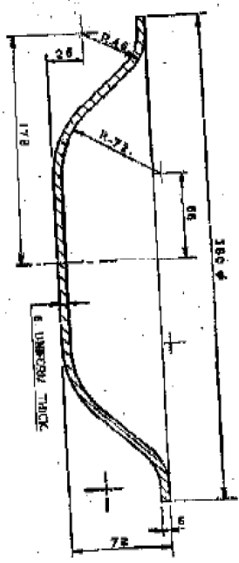
2" ODS. PUMP RUBBER DIAPHRAGM (CANVAS BRAIDED) SHEET - A. LEADERS: 72
