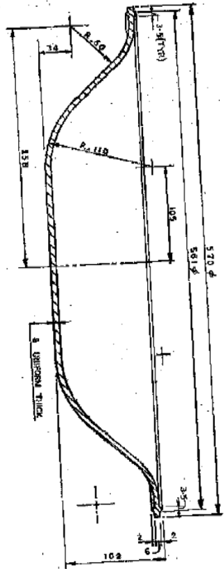
4" ODS. PUMP RUBBER DIAPHRAGM (CANVAS BRAIDED) SHEET - A. LEADERS: 55
