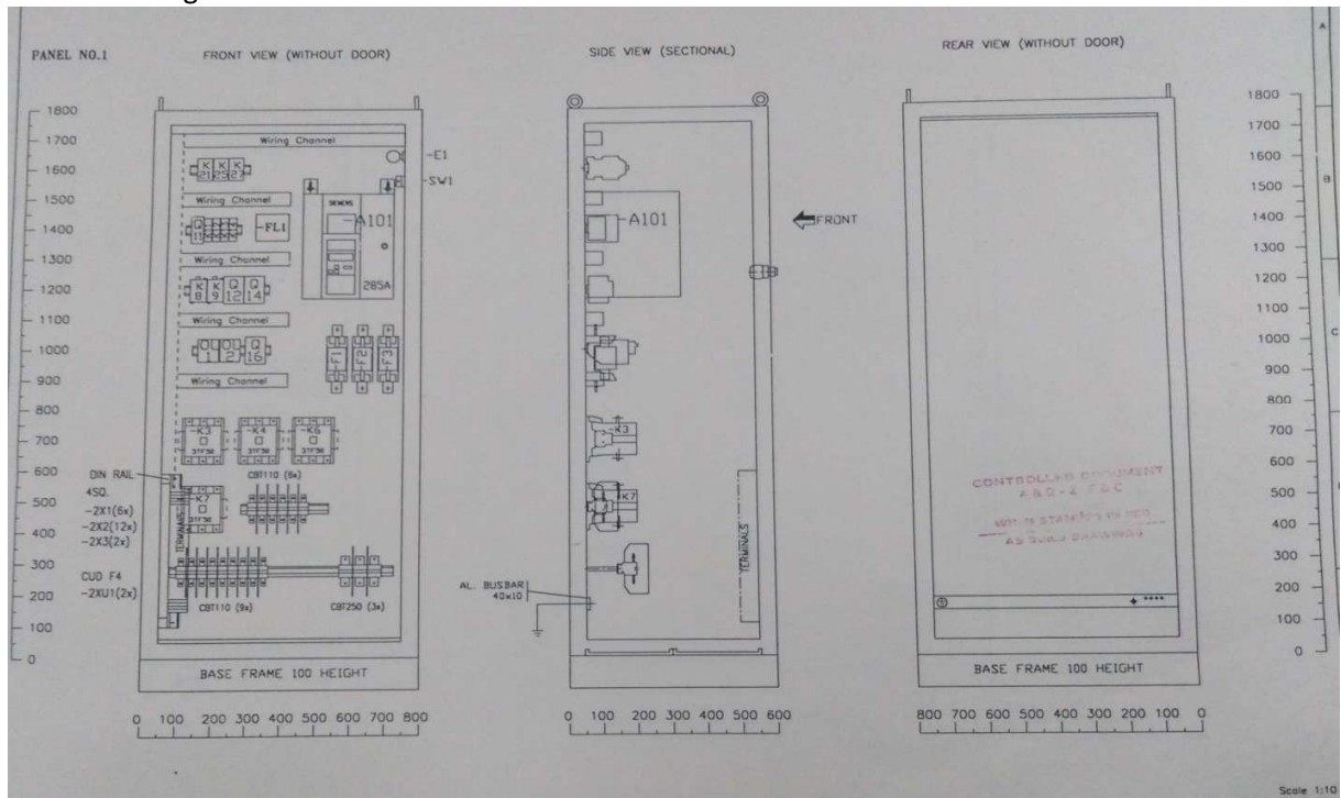
Figure 3- LT Panel
