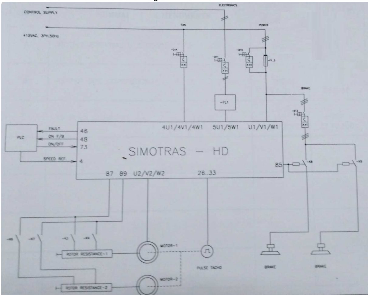
Figure 2 Single line Diagram
